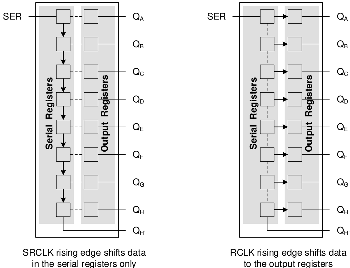
図 9-2. Simplified functional diagram showing clock operation
