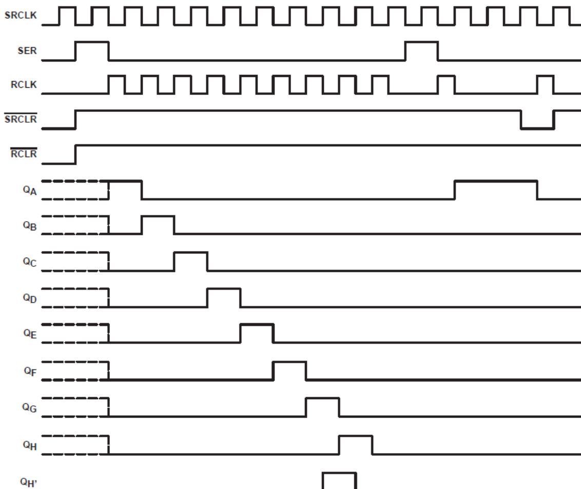
6-1. Timing Diagram
