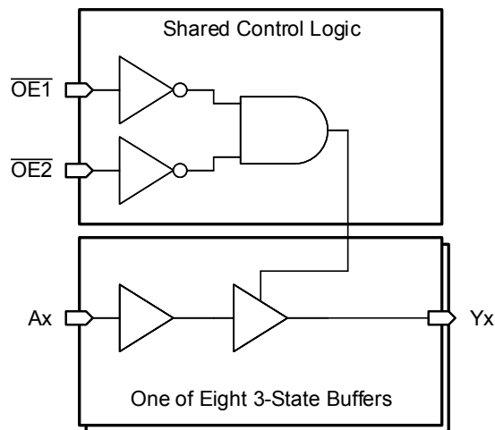
FIG 8-1. Logic Diagram (Positive Logic)
