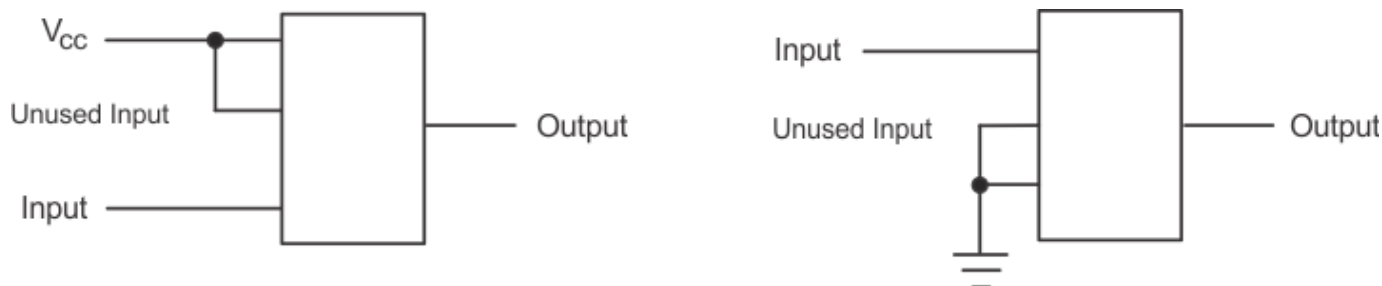
9-3. Layout Diagram
