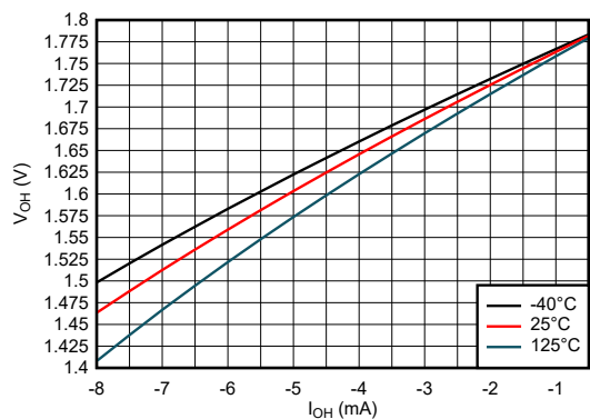
FIG 6-12. Output Voltage vs Current in HIGH State; 1.8-V Supply
