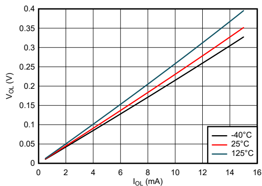
FIG 6-11. Output Voltage vs Current in LOW State; 2.5-V Supply
