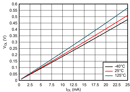
FIG 6-9. Output Voltage vs Current in LOW State; 3.3-V Supply
