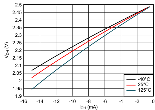
FIG 6-10. Output Voltage vs Current in HIGH State; 2.5-V Supply
