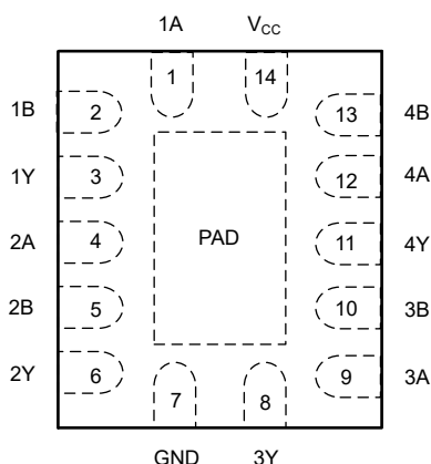
5-1. BQA Package, 14-Pin WQFN (Top View)
