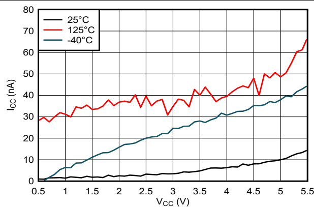
FIG 7-3. Supply Current Across Supply Voltage
