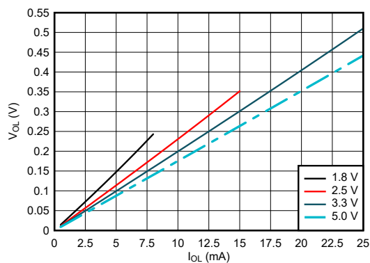
FIG 7-5. Output Voltage vs Current in LOW State
