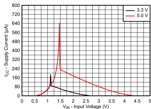
FIG 7-2. Supply Current Across Input Voltage 3.3-V and 5.0-V Supply
