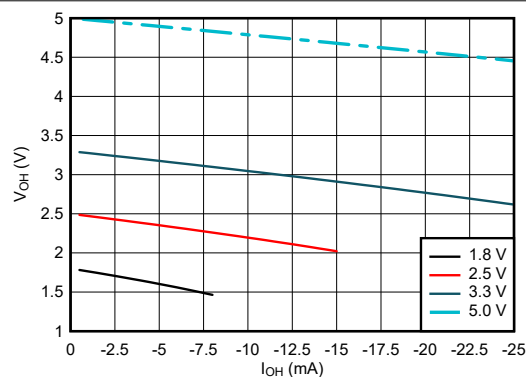
FIG 7-4. Output Voltage vs Current in HIGH State
