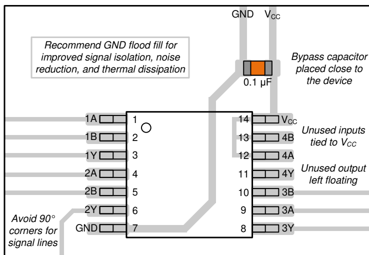
11-1. Example Layout for the SN74LV4T08
