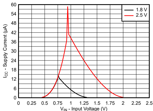
FIG 6-1. Supply Current Across Input Voltage 1.8-V and 2.5-V Supply
