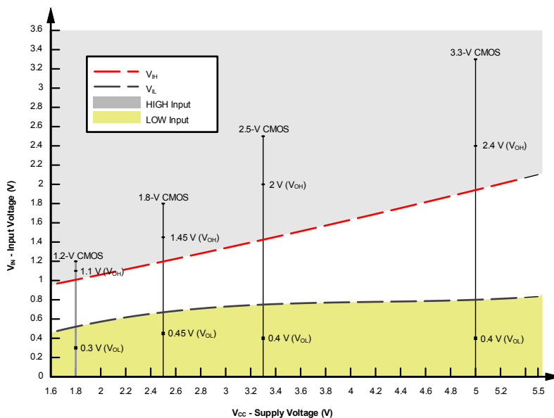
FIG 8-2. LVxT Input Voltage Levels
