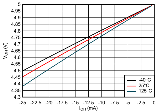
Figure 7-6. Output Voltage vs Current in HIGH State; 5-V Supply
