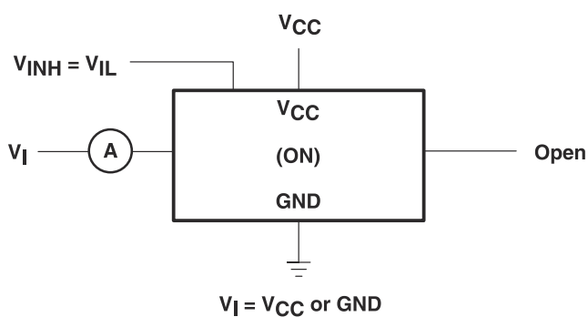
图 6-3. On-State Switch Leakage-Current Test Circuit
