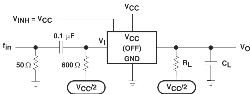
図 6-9. Feedthrough Attenuation (Switch Off)
