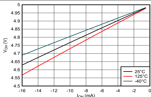
图 6-2. Output Voltage vs Current in HIGH State; 5-V Supply
