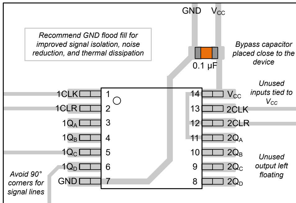
✎ 9-3. Layout Example for the SN74LV393B-EP in the PW Package
