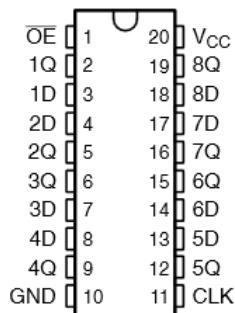
図 5-1. DB, DW, NS, or PW Package 20-PIN SSOP, SOIC, SO, or TSSOP (Top View)
