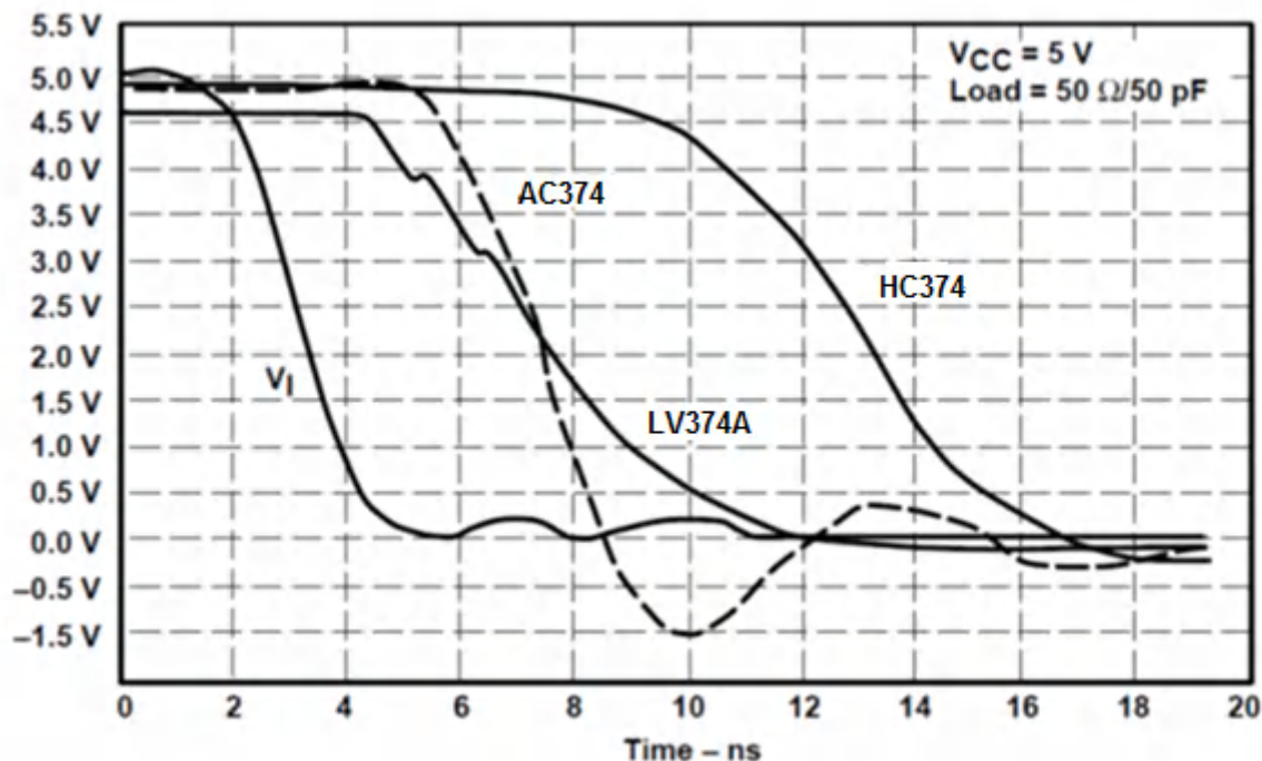
図 9-2. Switching Characteristics Comparison
