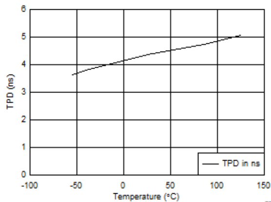
✎ 5-1. TPD vs Temperature at 5 V
