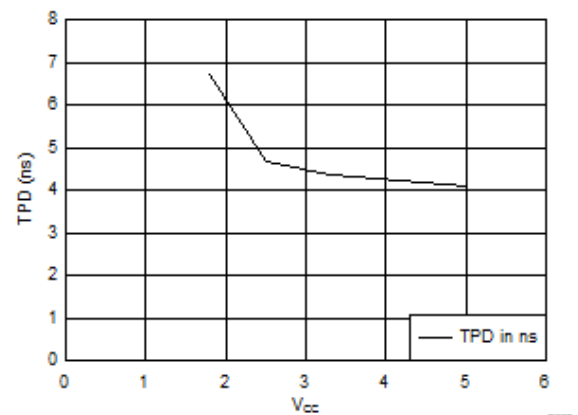
✎ 5-2. TPD vs V_{CC} at 25^\circ\text{C}
