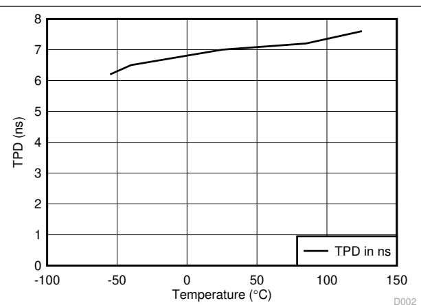
6-3. T_{PD} vs Temperature
