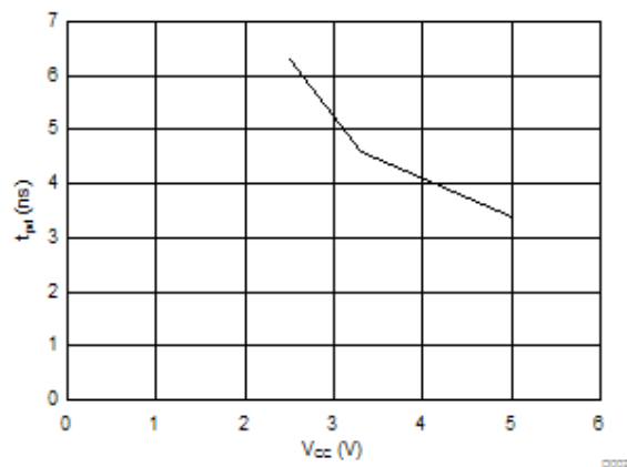
図 5-2. t_{pd} vs V_{CC} at 25°C
