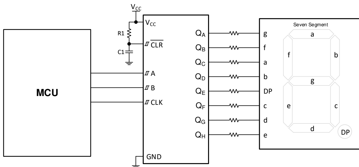
FIG 9-1. Typical Application Schematic
