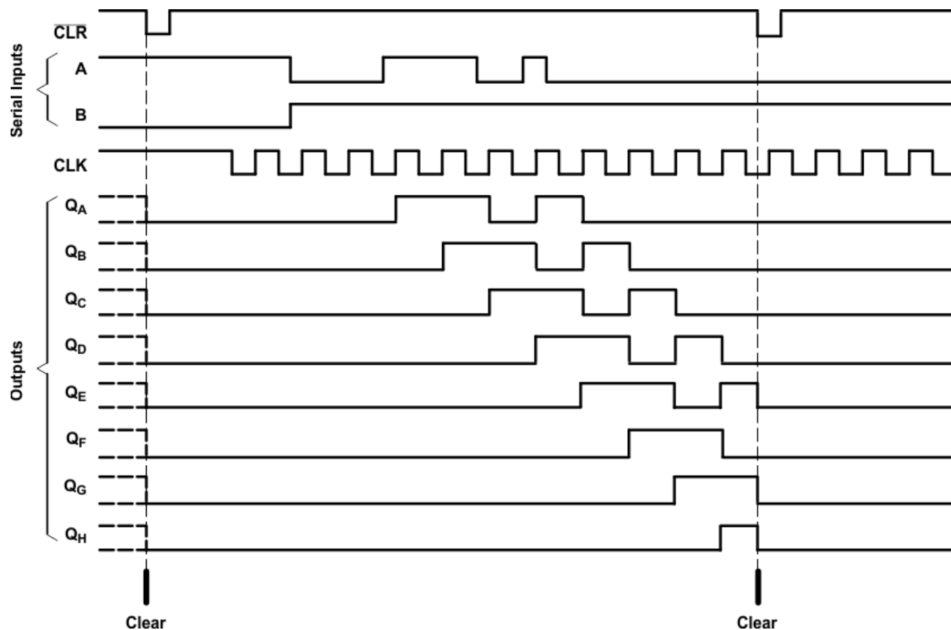
FIG 6-1. Typical Clear, Shift, and Clear Sequences
