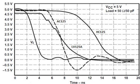
图 9-2. Switching Characteristics Comparison
