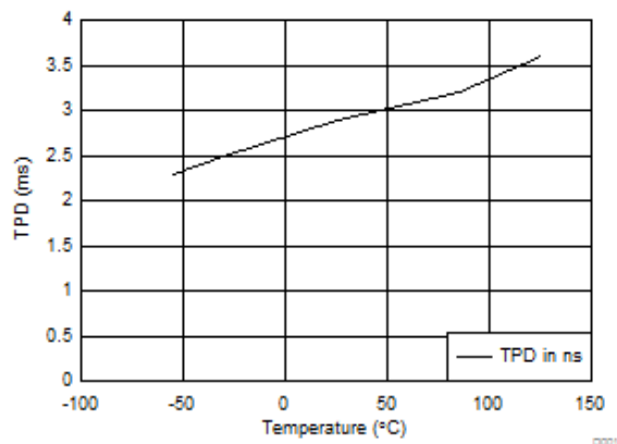
FIG 6-1. TPD vs Temperature at 5 V
