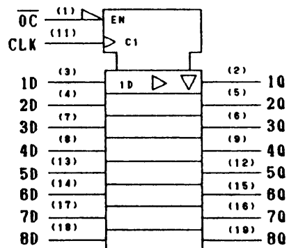
LOGIC SYMBOL
