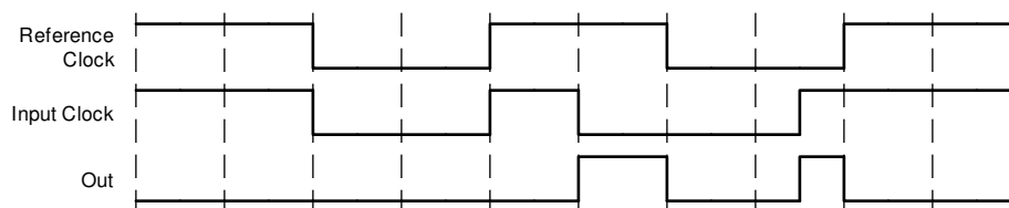
FIG 9-2. Application timing diagram
