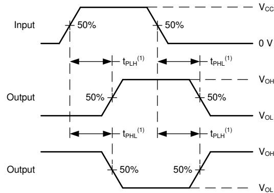
FIG 7. Voltage Waveforms Propagation Delays
