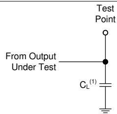
FIG 5. Load Circuit
