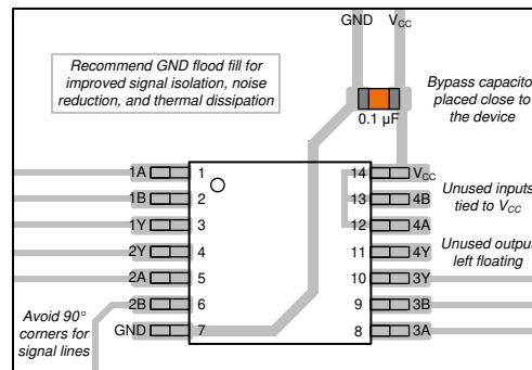
Figure 11. Example layout for the SN74HCS7266-Q1
