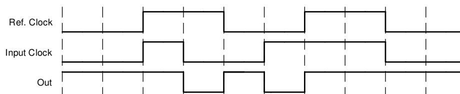
✕ 10. Application timing diagram
