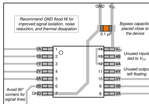
Figure 11. Example layout for the SN74HCS7266
