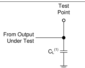
FIG 5. Load Circuit
