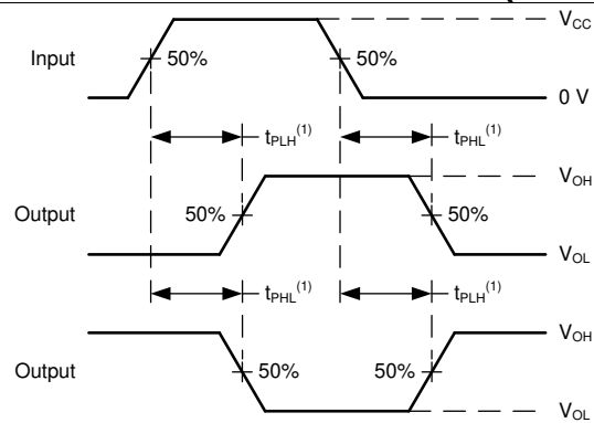
図 7. Voltage Waveforms Propagation Delays
