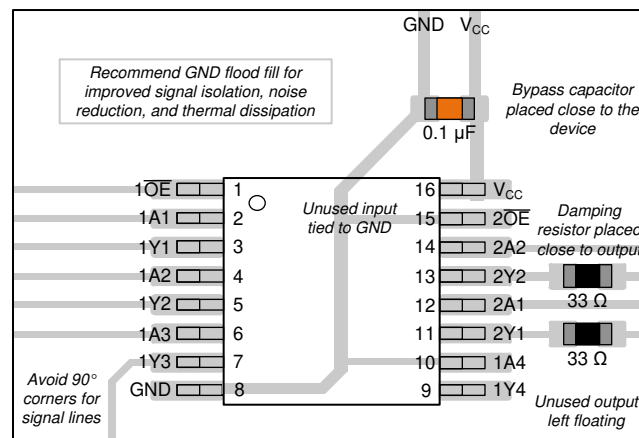
Figure 11-1. Example layout for the SN74HCS367 in the PW package.
