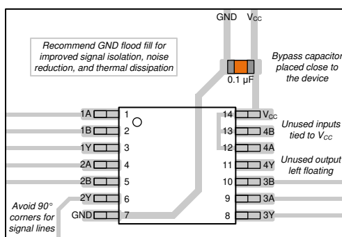
✎ 11-1. Example layout for the SN74HCS32
