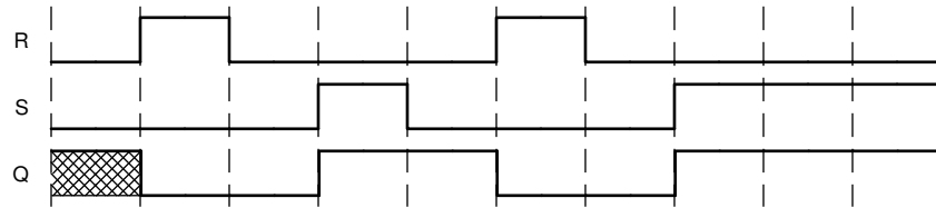
FIG 10. Application timing diagram
