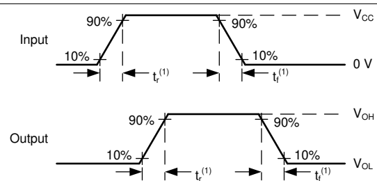
FIG 6. Voltage Waveforms Transition Times
