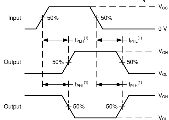
図 7. Voltage Waveforms Propagation Delays
