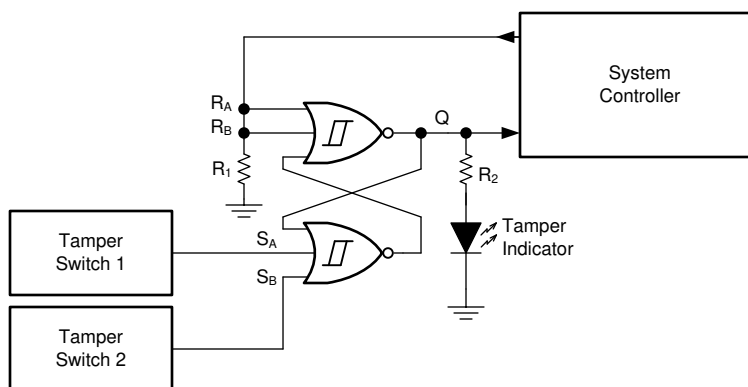
Figure 9. Typical application block diagram
