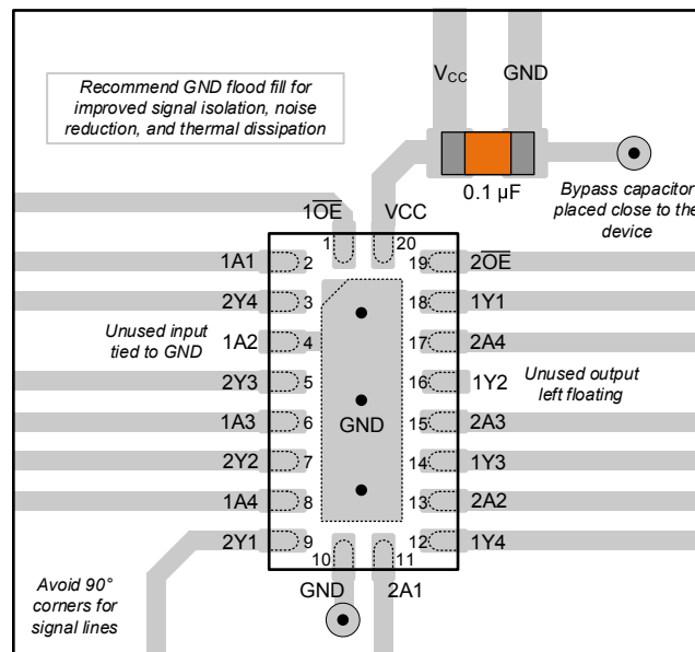
11-1. Example Layout for the SN74HCS240-Q1 in the WRKS Package
