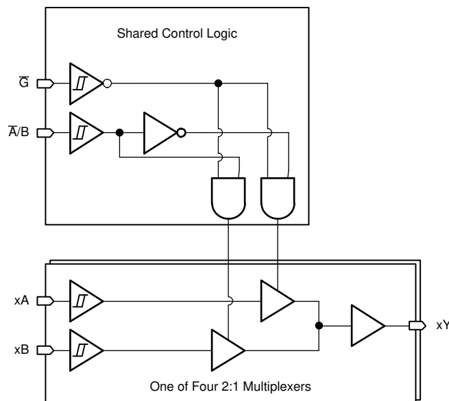
FIG 8-1. Logic Diagram (Positive Logic) for SN74HCS157-Q1
