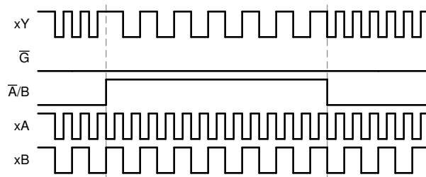
FIG 9-2. Application timing diagram
