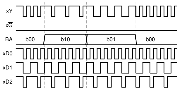
FIG 9-2. Application timing diagram
