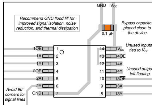
✎ 11-1. Example layout for the SN74HCS125
