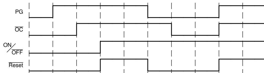
図 10. Application timing diagram
