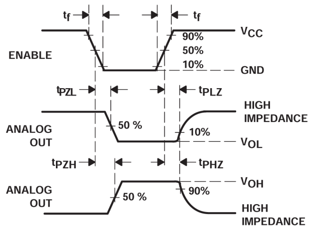
図 6-9. Propagation Delays, Enable to Analog Out
