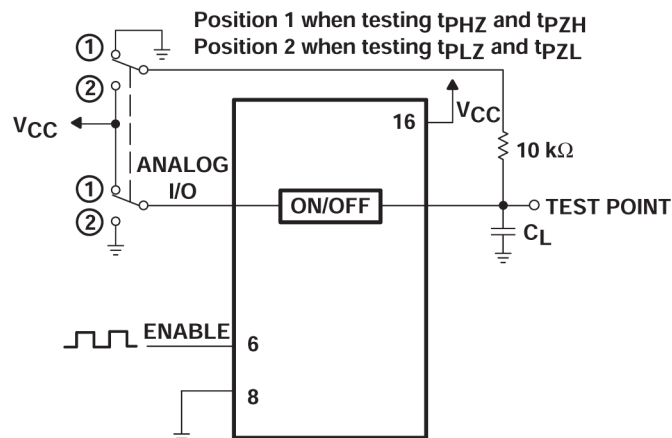
図 6-10. Propagation Delay, Enable to Analog Out, Test Setup
