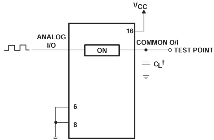
図 6-8. Propagation Delay, Analog in to Analog Out, Test Setup
