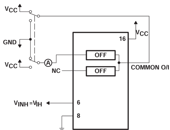
6-2. Maximum Off-Channel Leakage Current, Any One Channel, Test Setup
