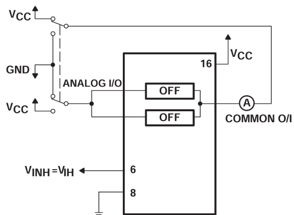
6-3. Maximum Off-Channel Leakage Current, Common Channel, Test Setup
