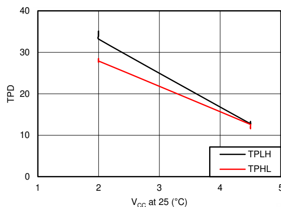
Figure 6-4. Typical propagation delay over supply ( V_{CC} at 25^\circ\text{C} )
