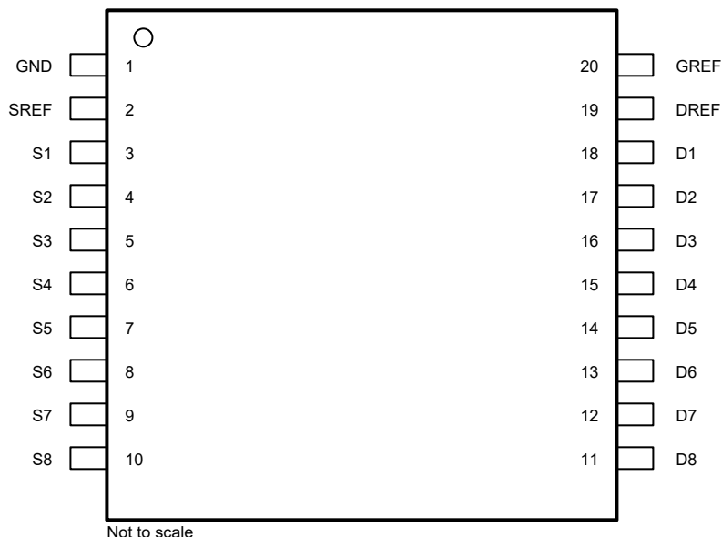
5-2. PW Package, 20-Pin TSSOP (Top View)
