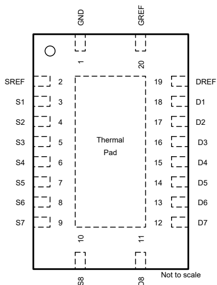
5-1. RKS Package, 20-Pin VQFN (Top View)
