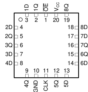
FIG 5-2. FK Package 20-Pin LCCC Transparent Top View
