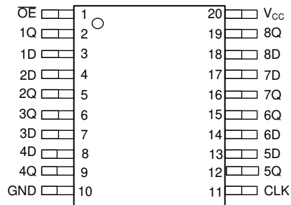
FIG 5-1. DB, DW, N, NS, J, or W Package 20-Pin SSOP, SOIC, PDIP, SO, CDIP, or CFP Top View
