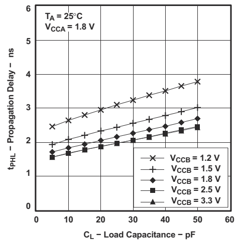
6-6. Typical Propagation Delay t_{PLH} (A to B) vs Load Capacitance
