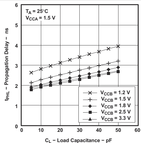
图 7-4. Typical Propagation Delay t_{PHL} (A to B) vs Load Capacitance
