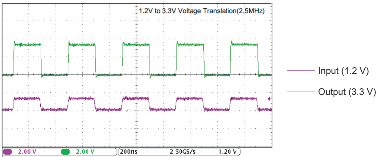
図 10-2. Translation Up (1.2 V to 3.3 V) at 2.5 MHz
