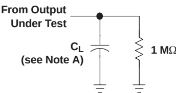
LOAD CIRCUIT
