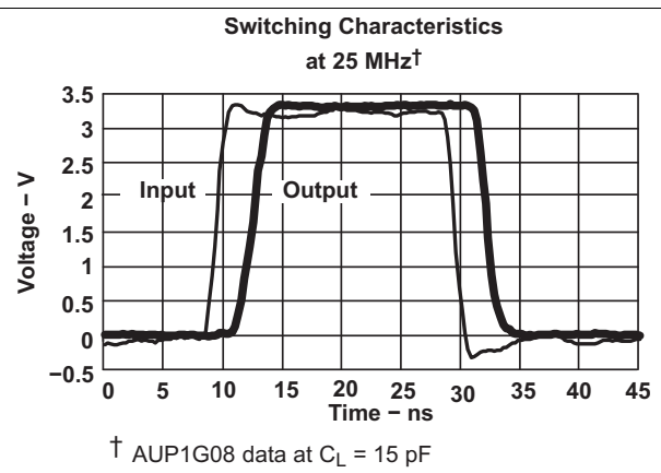
Figure 10. Excellent Signal Integrity
