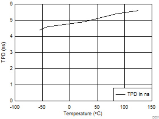
5-1. TPD vs Temperature
