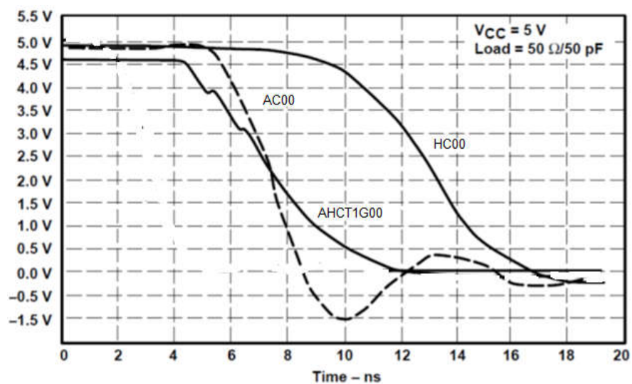
図 8-2. Switching Characteristics Comparison
