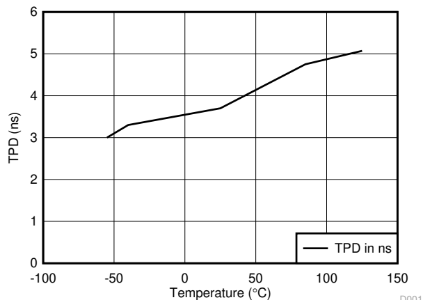
図 5-2. SN74AHC594 TPD vs Temperature, 15 pF Load RCLK to Q
