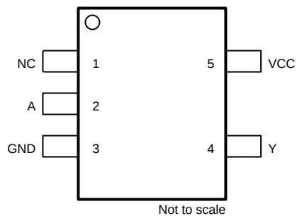
図 5-1. SN74AHC1G14-Q1 DBV Package, 5-Pin SOT-23; DCK Package, 5-Pin SC-70 (Top View)
