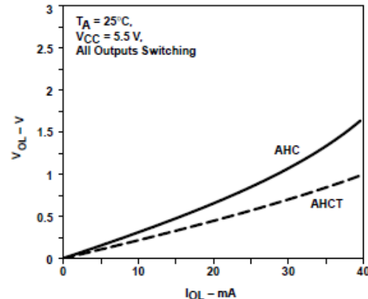
図 8-3. AHC Family V_{OL} vs I_{OL} at V_{CC} = 5.5 V
