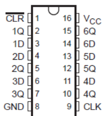
図 4-1. D, DB, DGV, N, NS, or PW Package (Top View)
