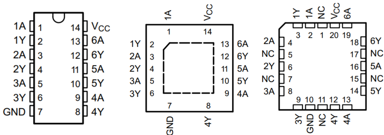
图 4-1. SN54AHC04 J or W Package SN74AHC04 D, DB, DGV, N, NS, or PW Package 图 4-2. SN74AHC04 RGY or BQA Package 图 4-3. SN54AHC04 FK Package (Top View) (Top View) (Top View)
