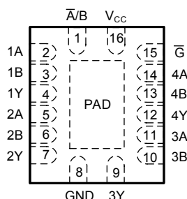
Figure 4-2. BQB Package, 16-Pin WQFN (Top View)
