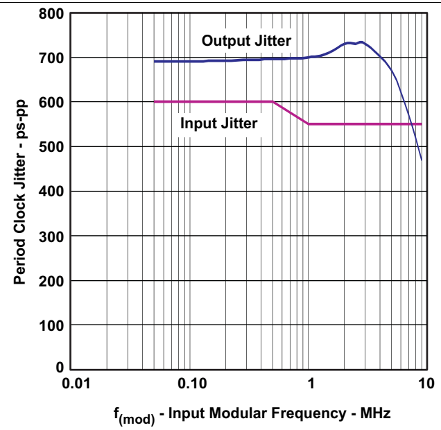
Figure 4. Output Clock Jitter vs Input Clock Jitter
