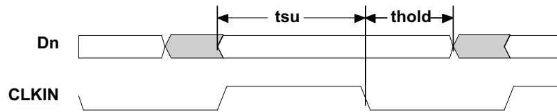
FIG 6. Set Up and Hold Time Definition
