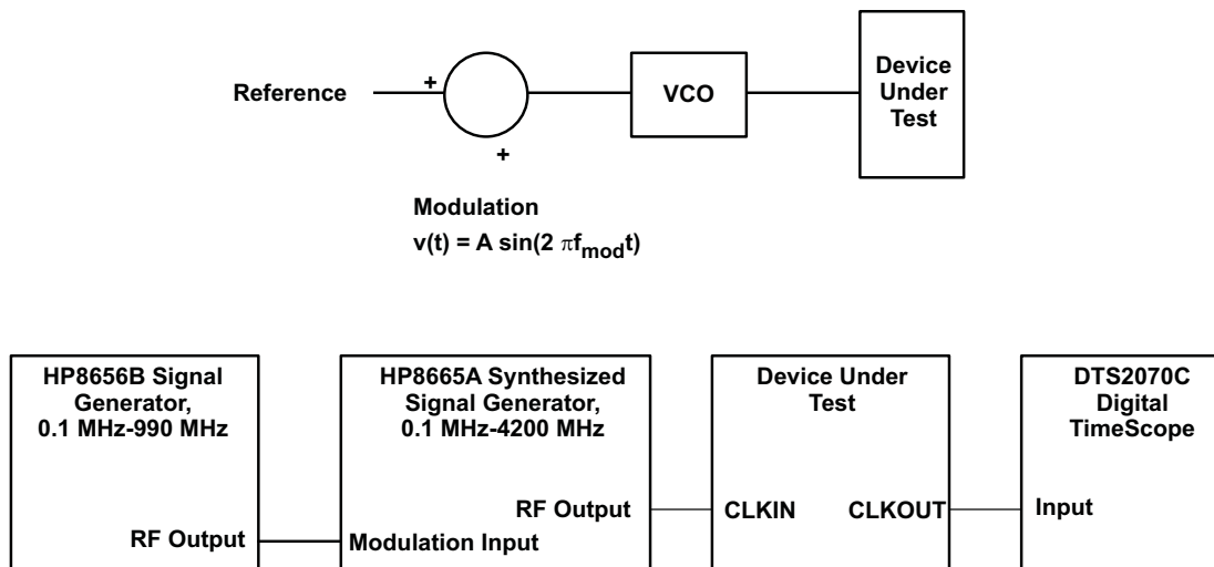
✎ 11. Output Clock Jitter Test Set Up
