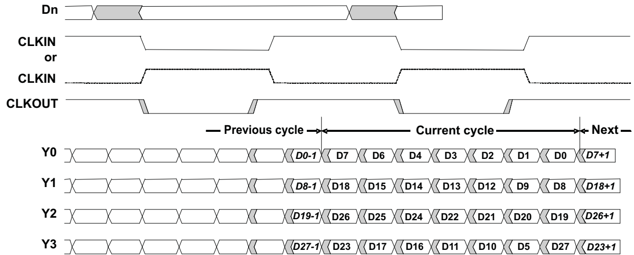
1. Typical SN65LVDS93A Load and Shift Sequences
