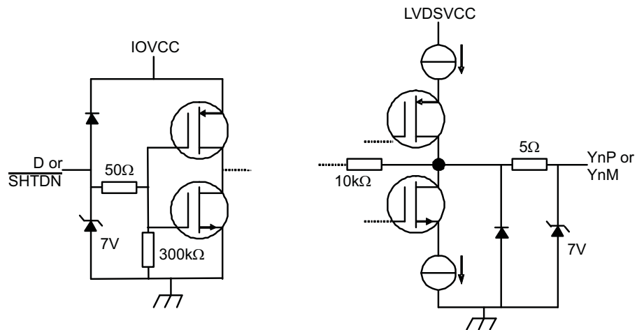
✎ 5. Equivalent Input and Output Schematic Diagrams
