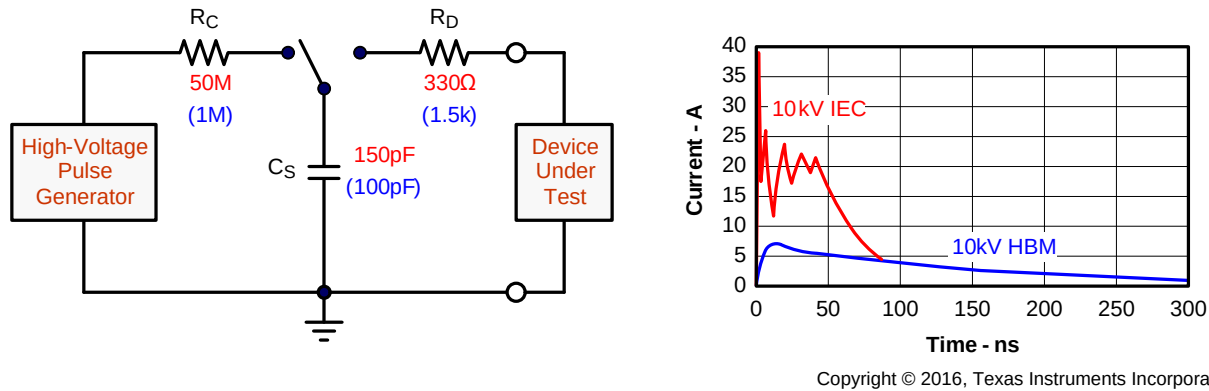
Figure 20. HBM and IEC-ESD Models and Currents in Comparison (HBM Values in Parenthesis)
