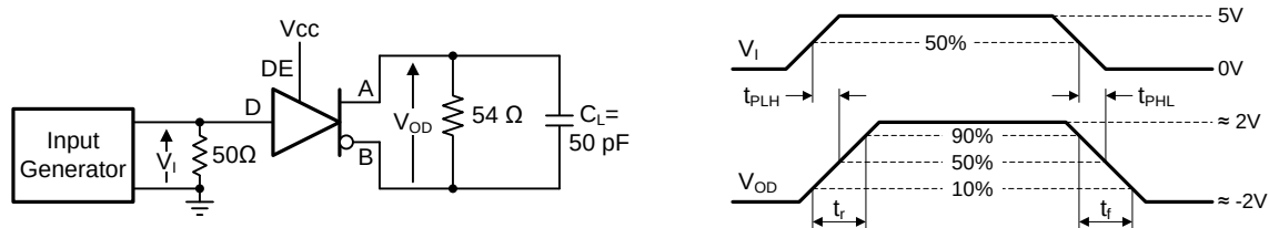
Figure 6. Measurement of Driver Differential-Output Rise and Fall Times and Propagation Delays
